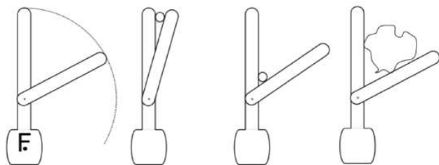
Figure 10.2.1: Simple 1-DoF grasping mechanism that relies on friction to grasp objects with a wide variety of sizes (center, right). The mechanism has only one moving part that presses the object against a passive finger.
